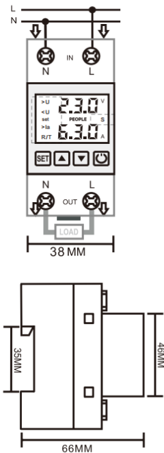
●Wiring diagram/Dimensional Drawing
