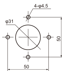
outside operation mounting baseplate
