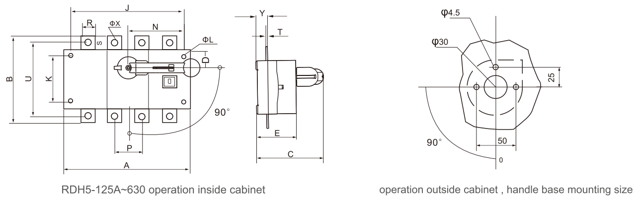
RDH5(HGL)-125A~630A direct operation
