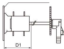
outside cabinet operation mounting baseplate
