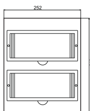
DB124/FT 24 ways
