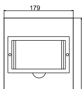
DB108/F 8 ways
