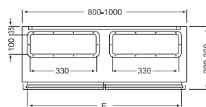
Section through y-y with door open
