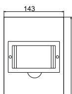
DB106/F 6 ways
